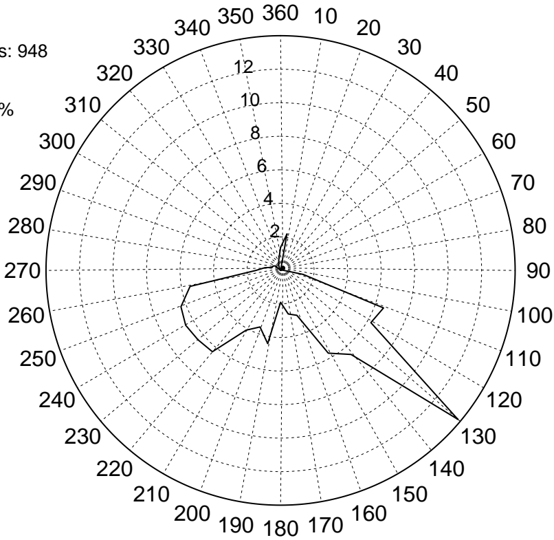
Frequency of wind direction (%)
