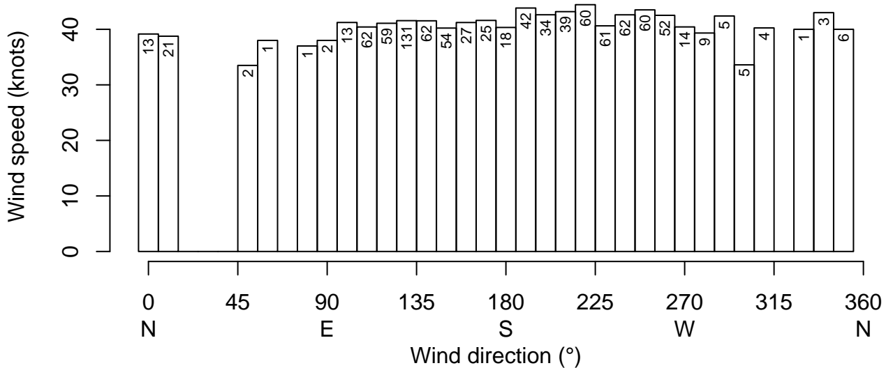
(Number of observations for wind direction)
