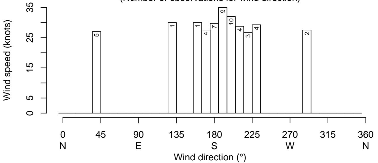
(Number of observations for wind direction)
